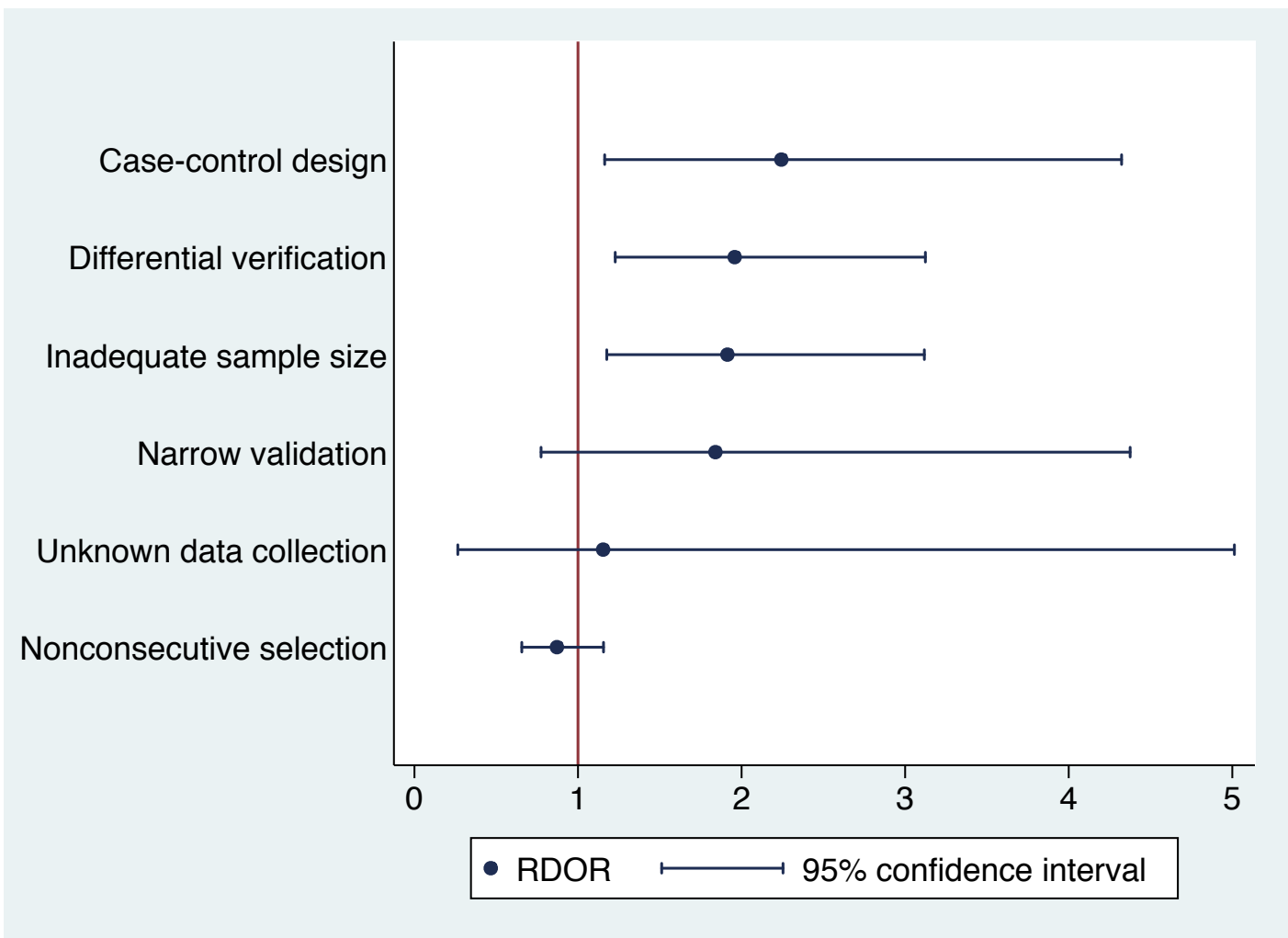
Figure 1. Multivariable analysis: influence of design deficiencies on the performance of clinical prediction rule under random-effects assumption between meta-analyses.
